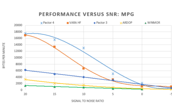
PACTOR 4 was the clear leader in the MPG case with VARA in a respectable second place. WINMOR would not pass traffic reliably at -a 5dB SNR.
